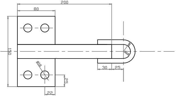
SE001 Roof Anchor Plan Scale 1:1
