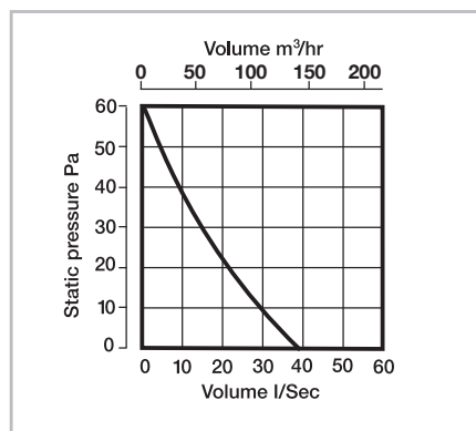
Performance - 125mm Frame Fan
