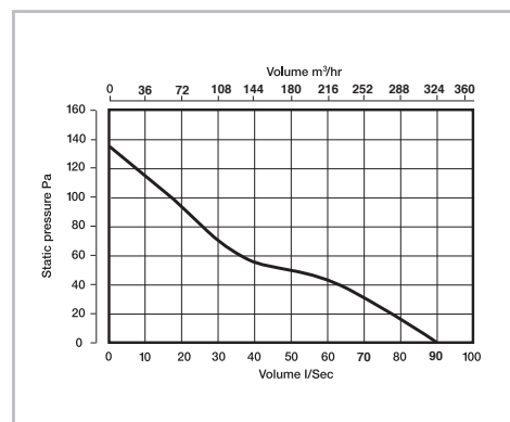
Performance - 150mm Frame Fan
