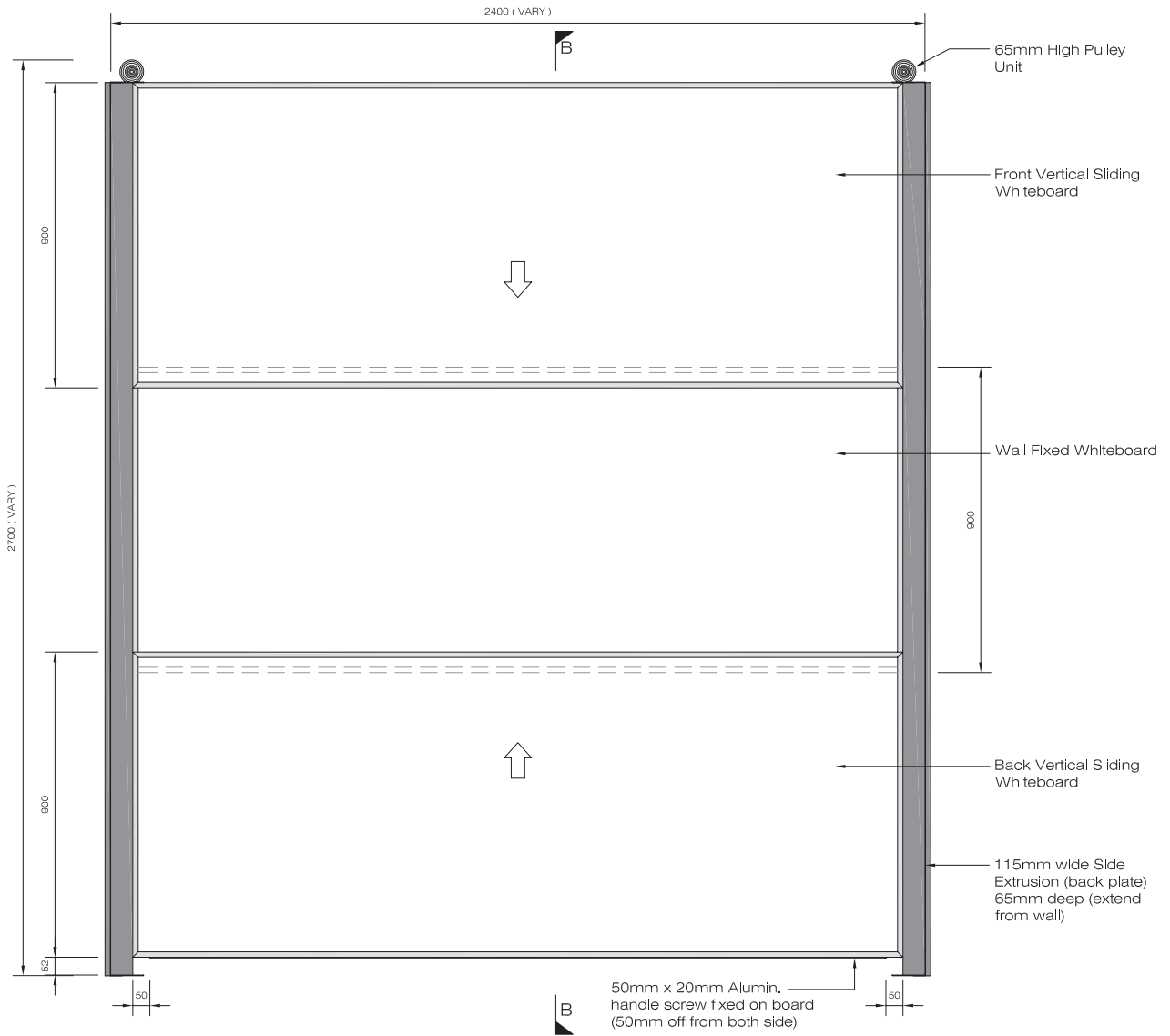
Front elevation - (Counterweight)
