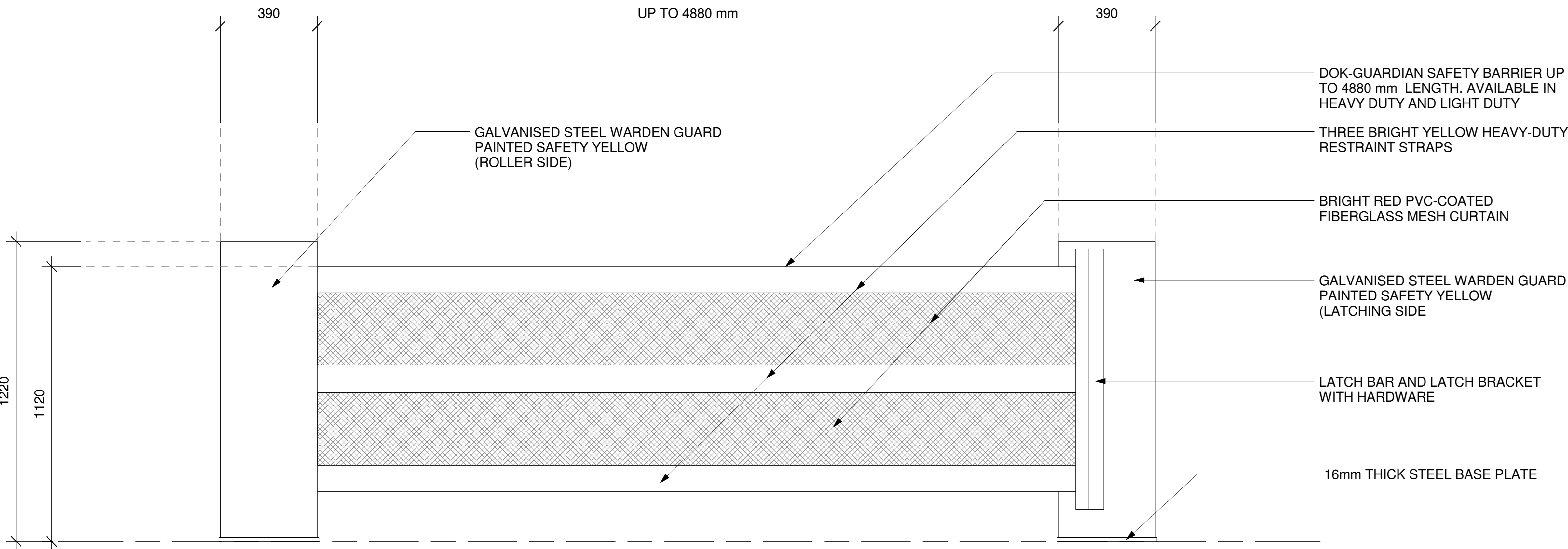
ELEVATION VIEW SCALE: 1:10 MTS.
