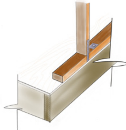
Strap/M12 Bolt Connection to Timber
