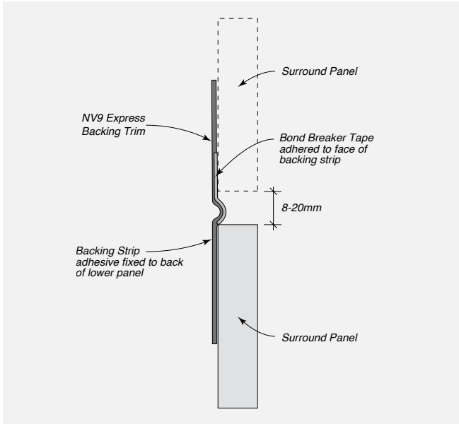
FIGURE 7.16 Horizontal Joint Sealed Side
