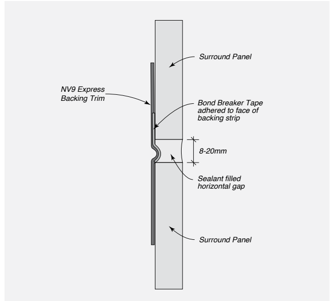
FIGURE 7.19 Horizontal Joint Sealed Side
