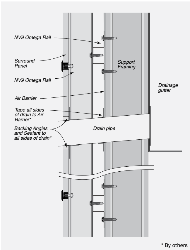
FIGURE 8.23 Typical Penetration
