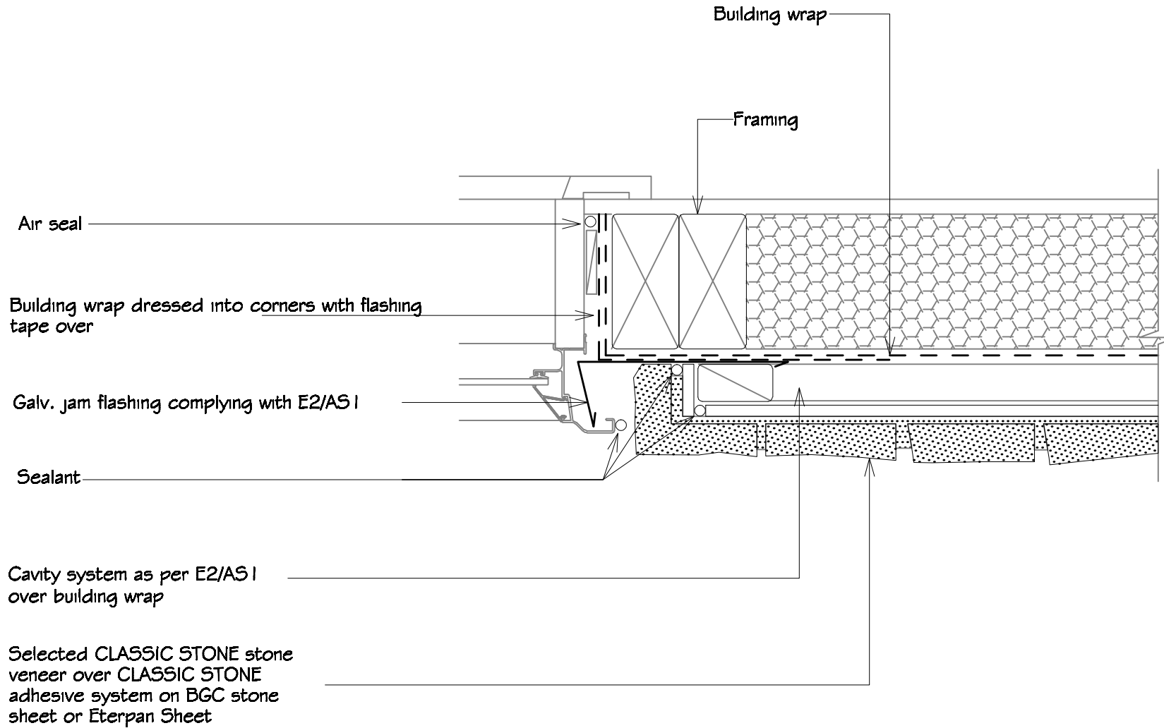
4a - Typical Window Jamb Detail - Recessed (plan view)
