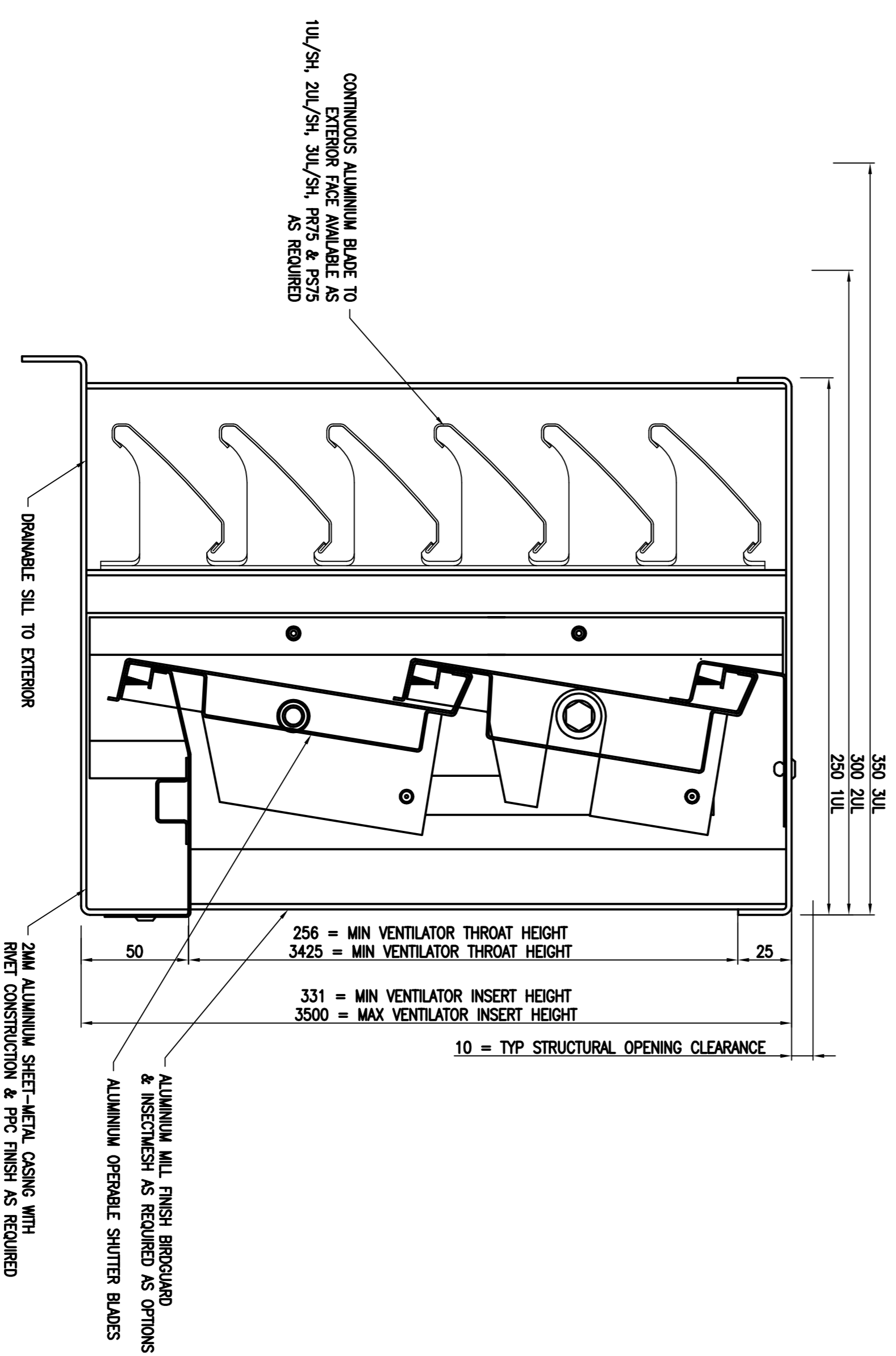
CROSS SECTIONAL END VIEW OF UOL A1: SCALE 1:2
