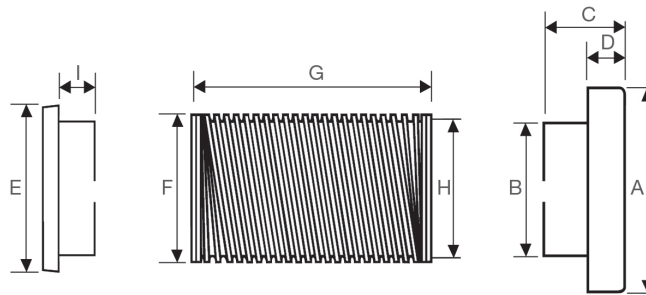
Dimensions - XPS230/300
