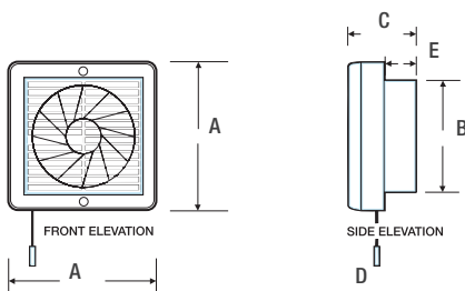
Dimensions - XFS230/300
