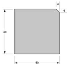
SISCS Internal Corner Board 40mm x 40mm
