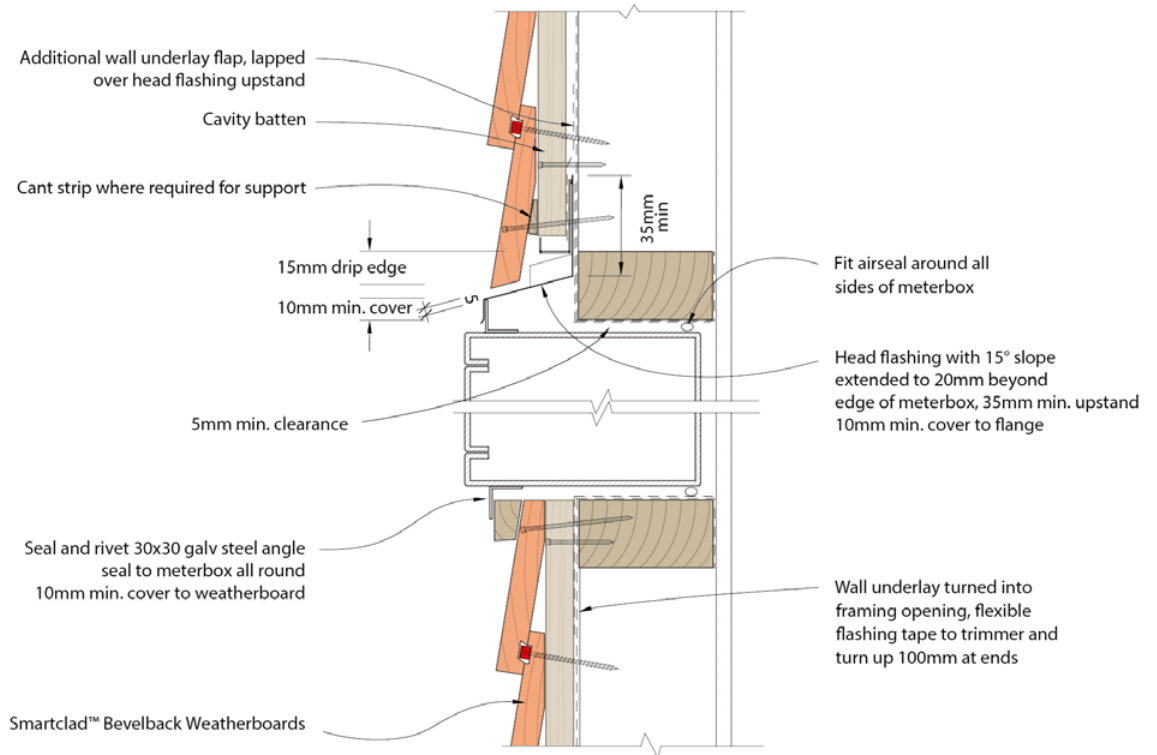
Figure 16: Bevelback — Meter Box Head & Sill
