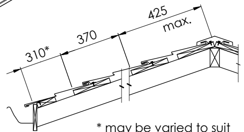
Batten Detail
