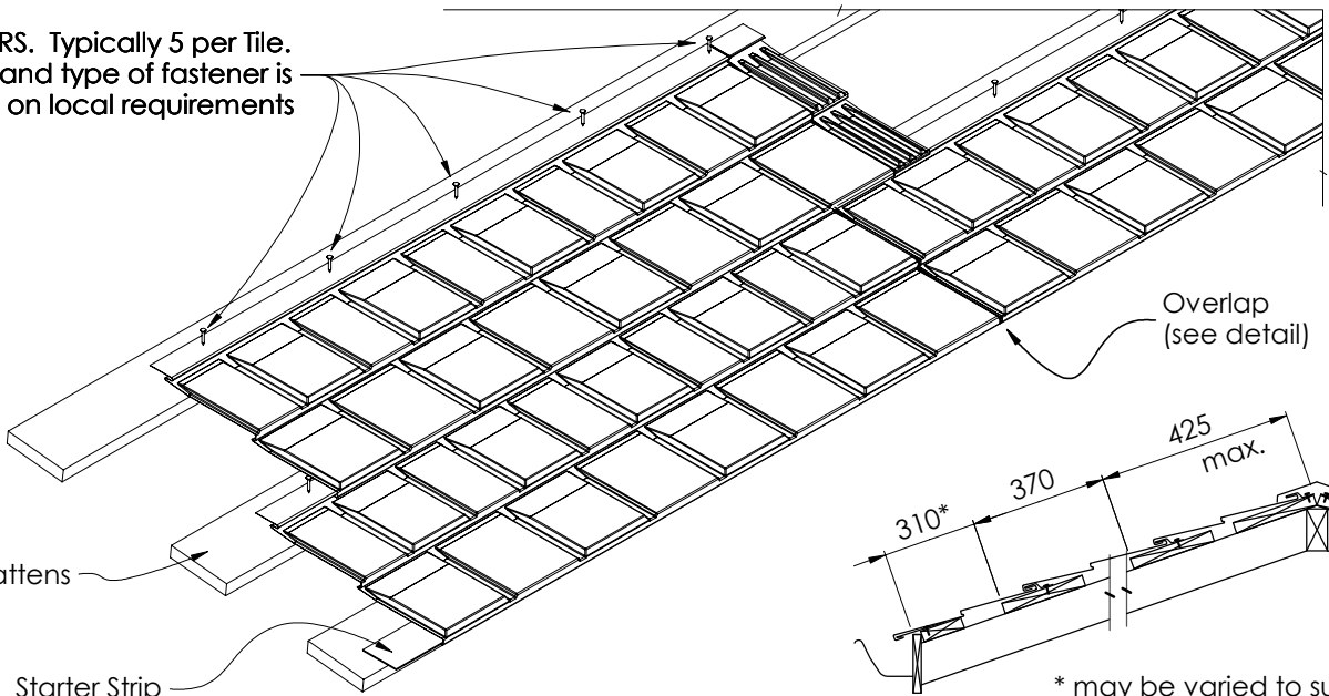
Fastening Detail
