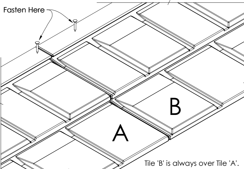
Overlap Detail
