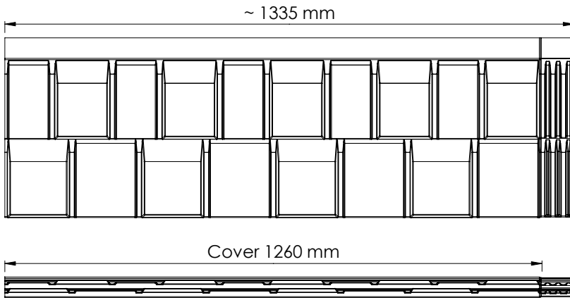
Tile Dimensions
