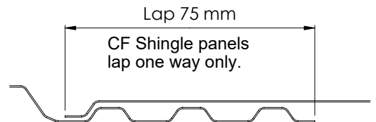
Figure 12.4 Side Lap Detail
