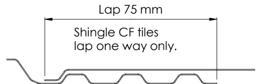
Side Lap Detail
