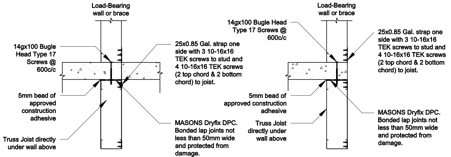
INTERNAL WALL ABOVE JOIST 6kN CONNECTOR DETAIL 11 Scale 1:10
