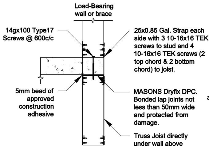
EXTERNAL WALL ABOVE JOIST 12kN CONNECTOR DETAIL 8 Scale 1:10
