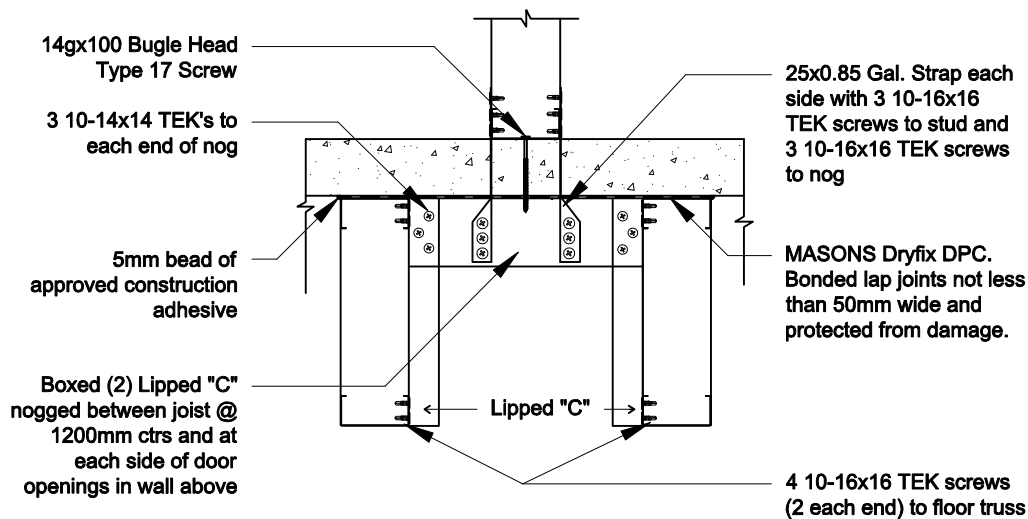
INT/EXTERNAL WALL 12kN CONNECTOR OVER NOG DETAIL 10 Scale 1:10
