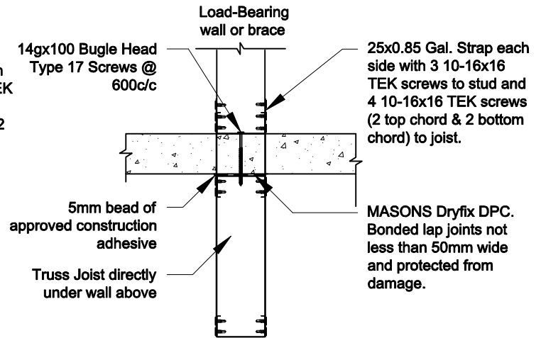
INTERNAL WALL ABOVE JOIST 12kN CONNECTOR DETAIL 9 Scale 1:10
