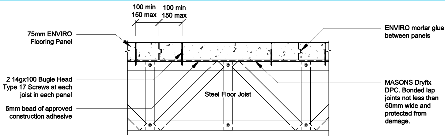
TYPICAL PANEL INSTALLATION DETAIL 5 Scale 1:10
