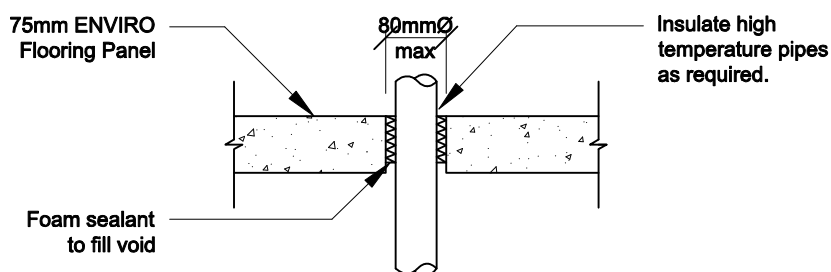
TYPICAL PENETRATION DETAIL 6 Scale 1:10
