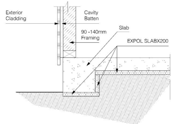
Slab on Grade with Footing 90 -140mm Framing/Cladding
