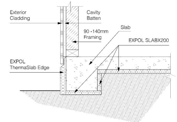
Slab on Grade with Footing 90 -140mm Framing/Cladding
