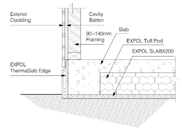
Waffle Pod Floor 90 -140mm Framing/Cladding
