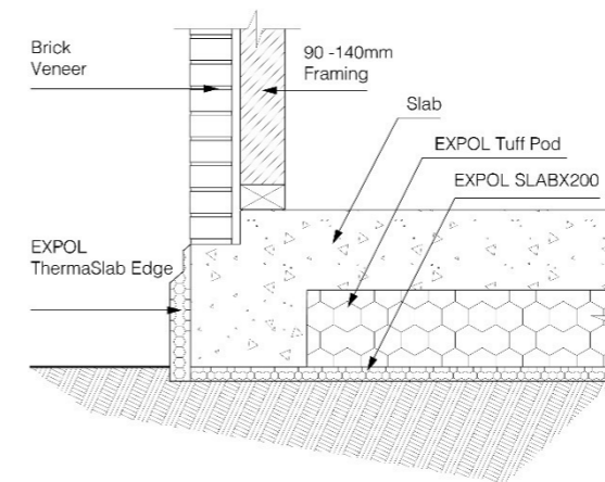
Waffle Pod Floor 90 -140mm Framing/Brick Veneer
