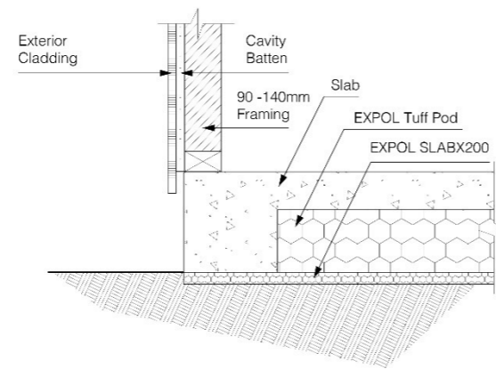
Waffle Pod Floor 90 -140mm Framing/Cladding
