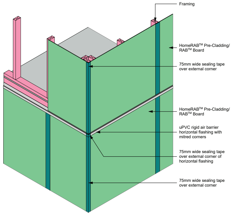
Figure 14c: Corner junction to horizontal joint
