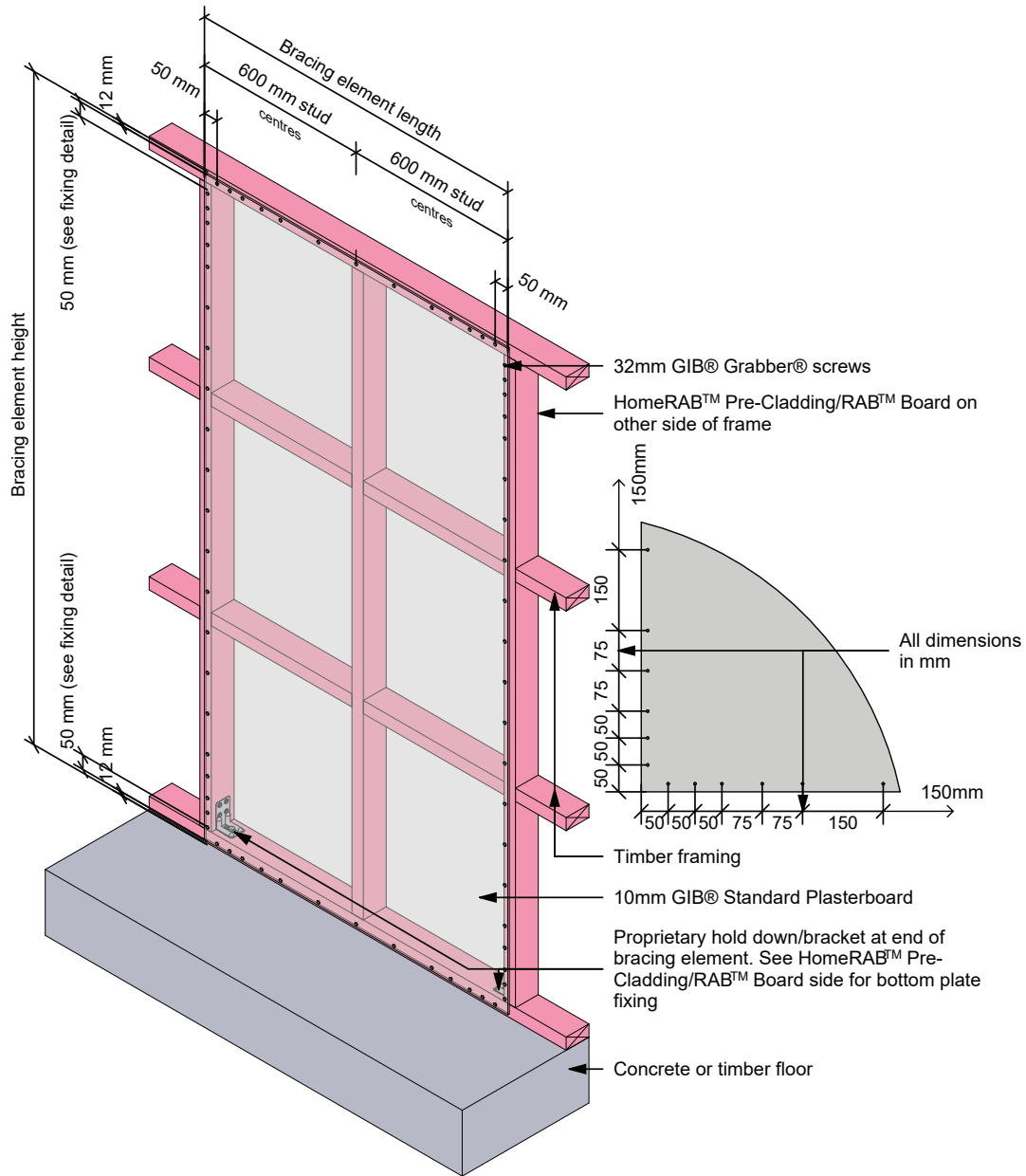
Figure 34: 1200mm HomeRAB™ Pre-Cladding with 10mm GIB® Standard Plasterboard
