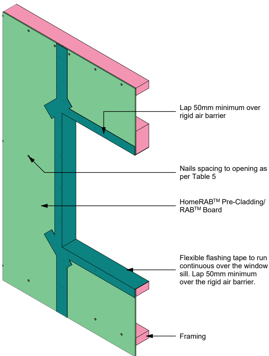
Figure 19: Window sealing with flashing tapes
