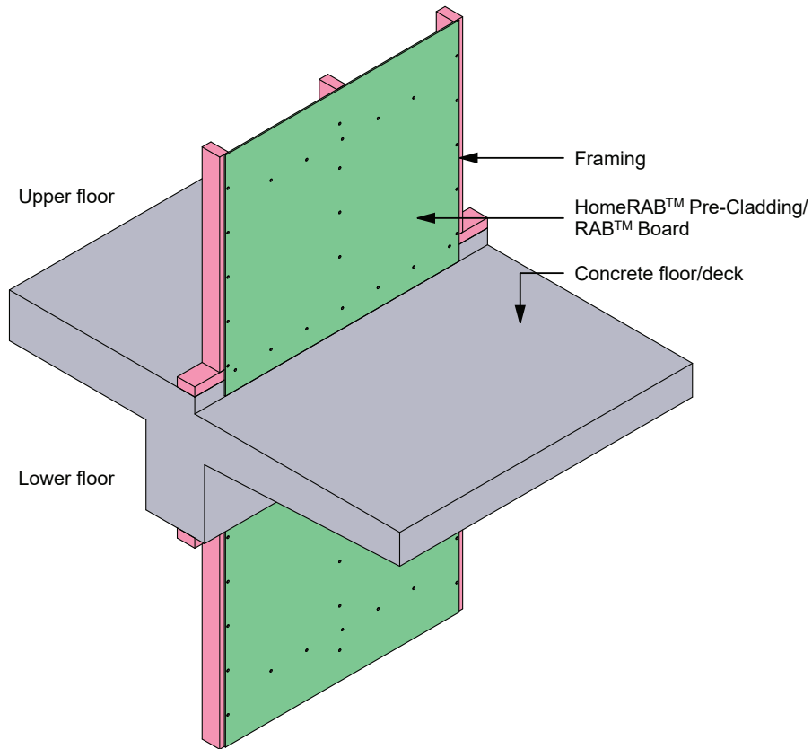
Figure 22: RAB™ Board to concrete slab junction
