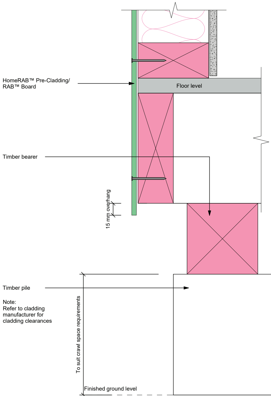
Figure 7: Foundation detail – timber pile foundation
