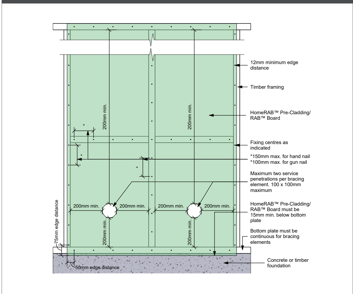
Figure 27: Penetrations in Bracing Sheet
