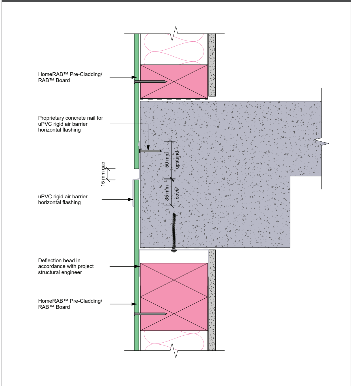
Figure 26: Deflection head
