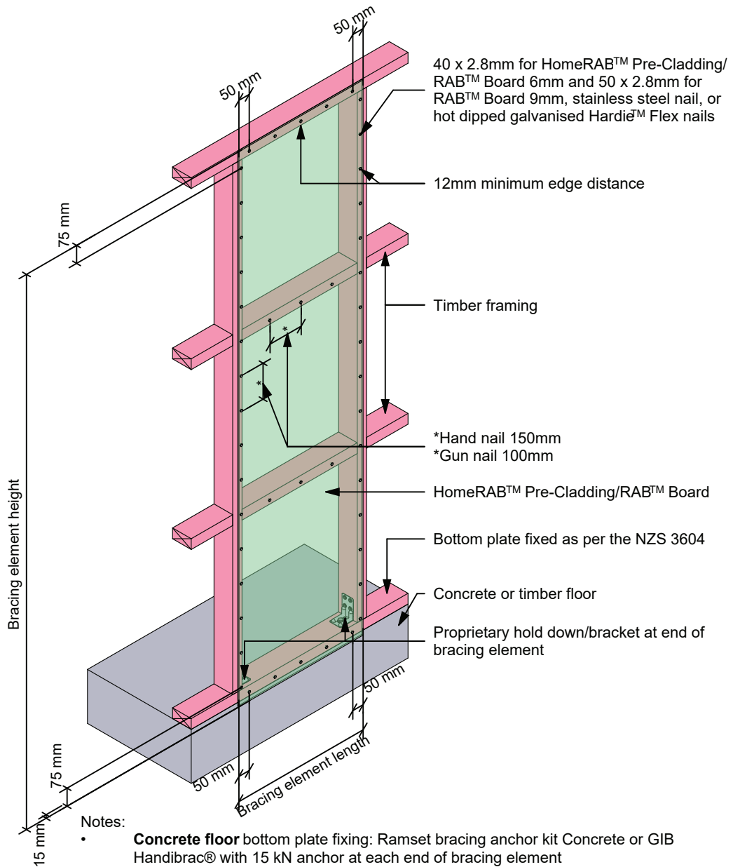
Figure 29: 400/600mm HomeRAB™ Pre-Cladding or RAB™ Board to concrete or timber floor
