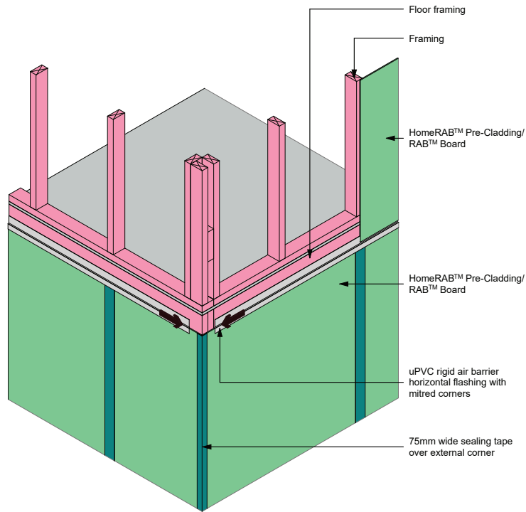
Figure 14a: Corner junction to horizontal joint
