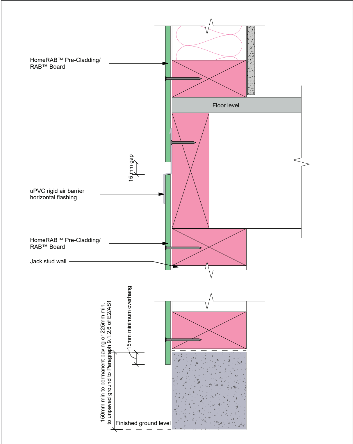
Figure 6: Foundation detail – timber foundation
