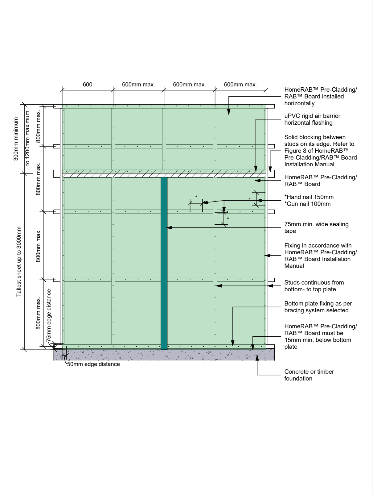
Figure 35: Sheet layout for tall walls up to 4.2m
