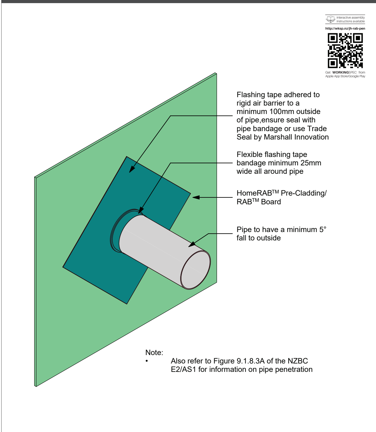
Figure 23: Pipe penetration through HomeRAB™ Pre-Cladding and RAB™ Board
