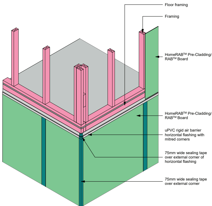
Figure 14b: Corner junction to horizontal joint
