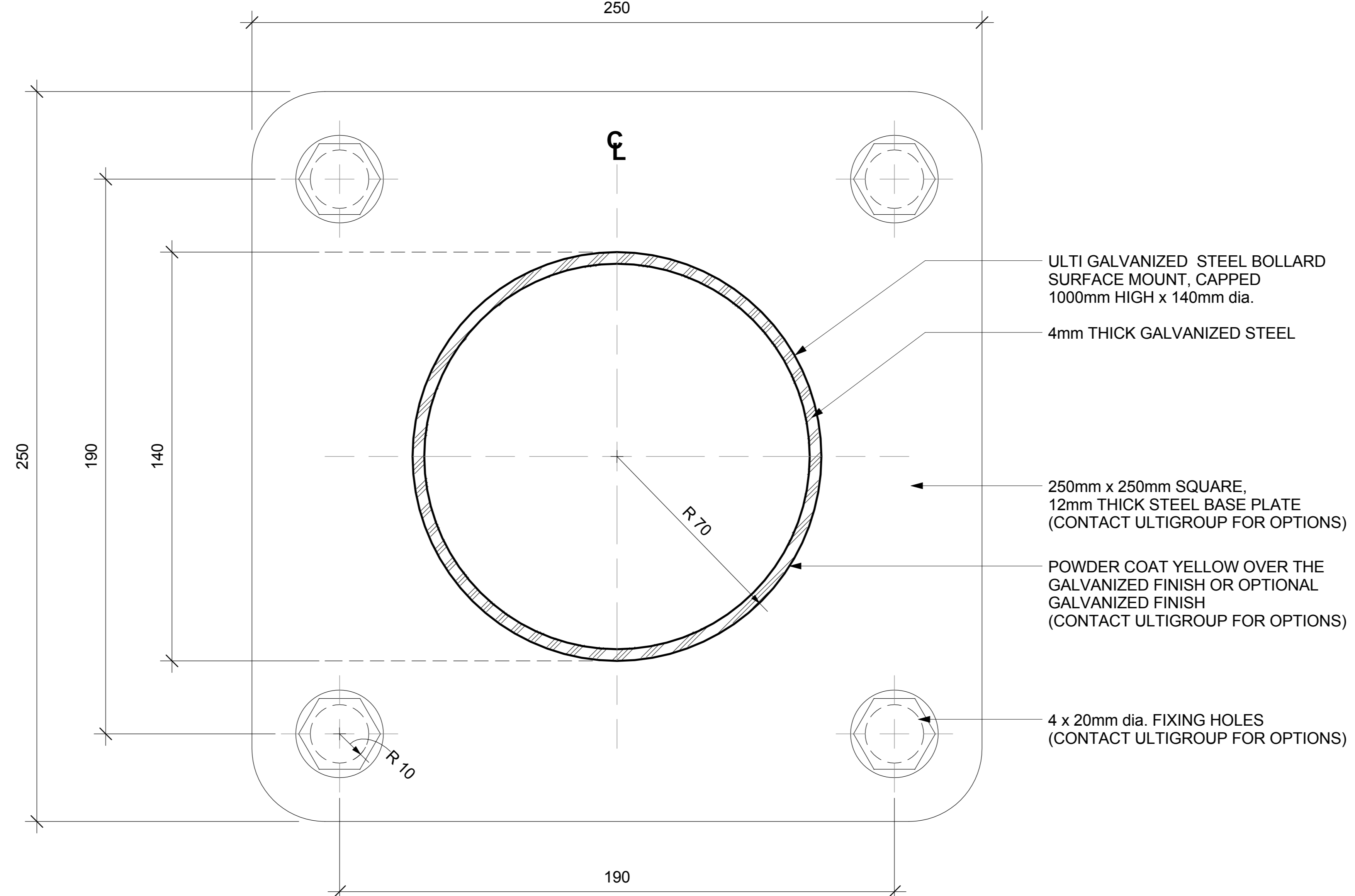
3 PLAN - SURFACE MOUNT BOLLARD SCALE: 1:1 MTS.
