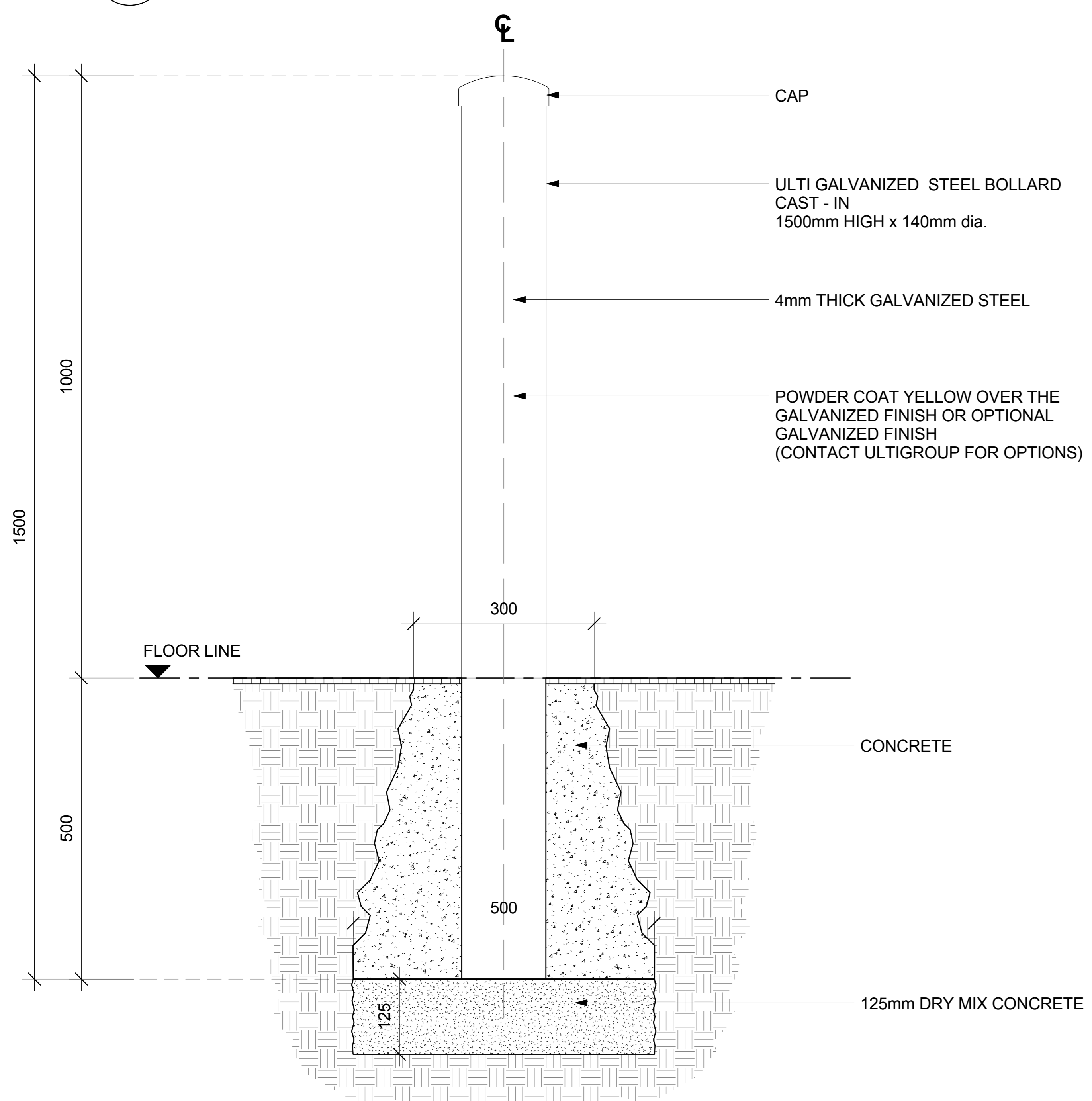
2 ELEVATION - CAST IN BOLLARD SCALE: 1:5 MTS.
