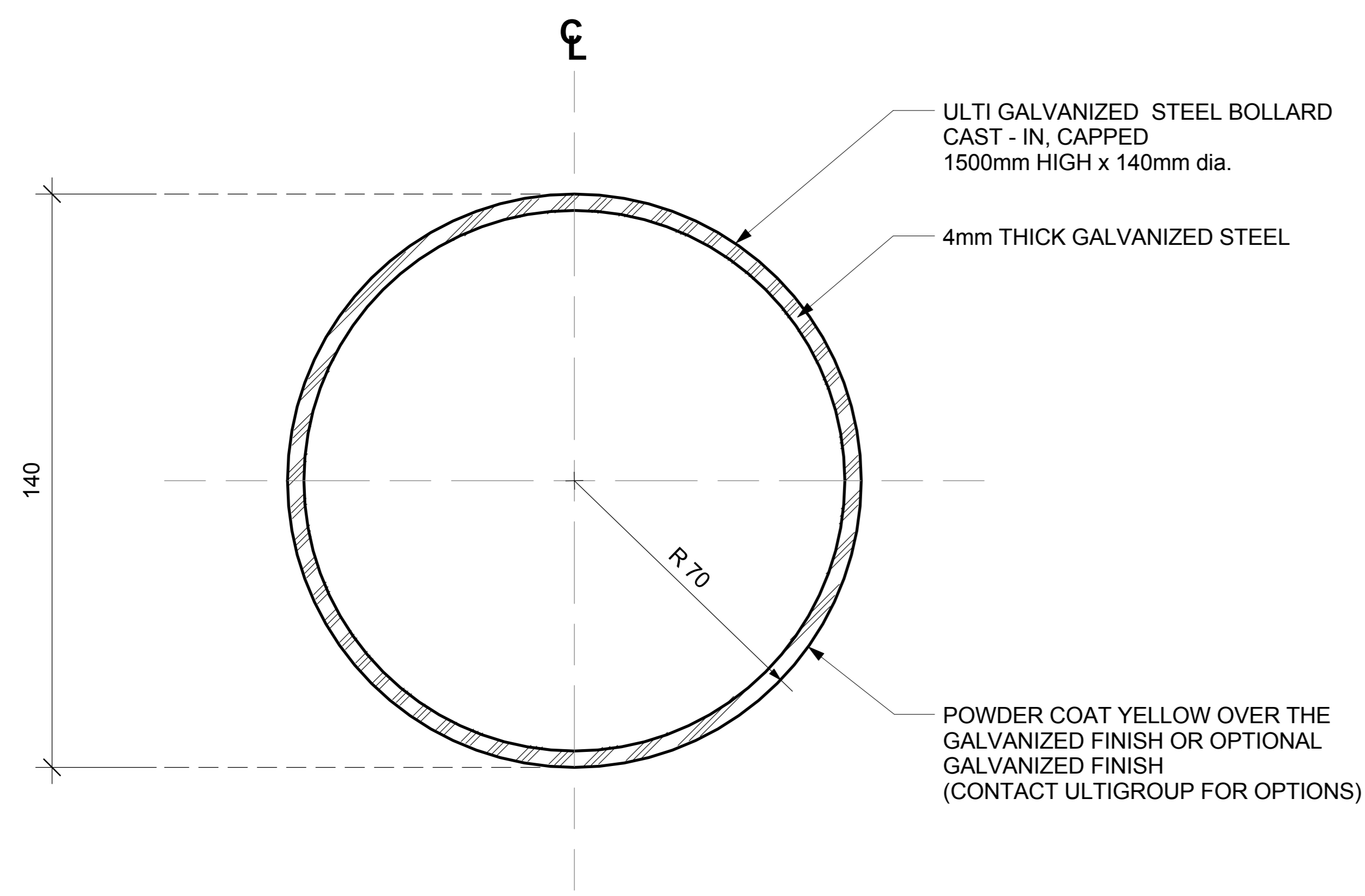
1 PLAN - CAST IN BOLLARD SCALE: 1:1 MTS.
