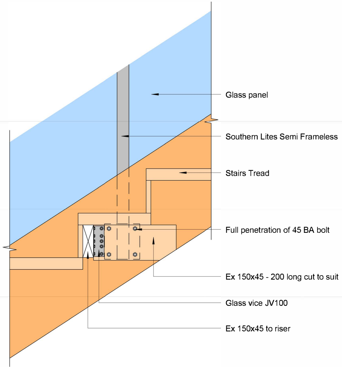
2 Section Detail View C-C 1 : 10
