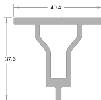
FACE FIX EDGE POST STIFFENER JEB/205/5
