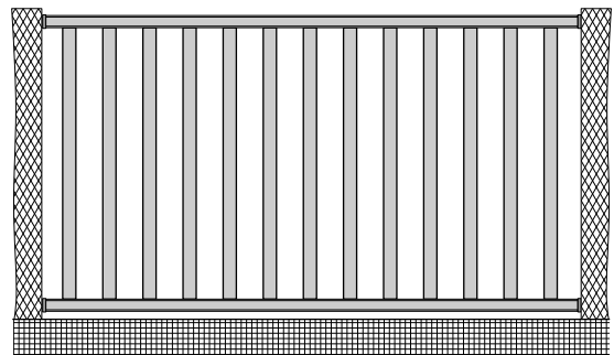
Infill Slat 49mm JVB/018 Gaps 99mm max
