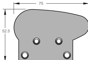
HANDRAIL WALL ATTACH END PLATE Part No JEC217/WC
