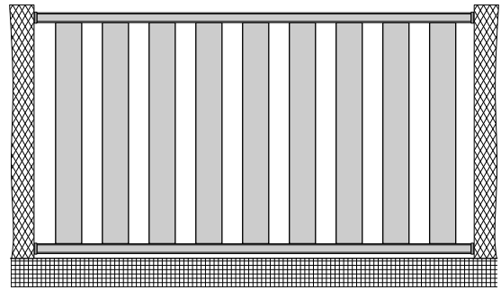
Infill Slat 123mm JGF/2227. Gaps 99mm max
