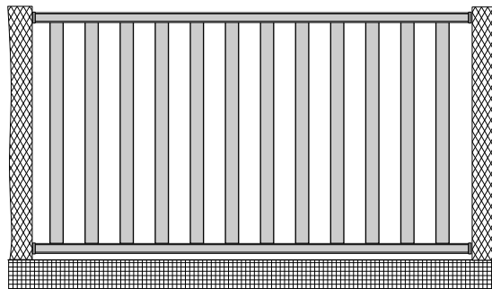
Infill Slat 60mm JVB/019 Gaps 99mm max
