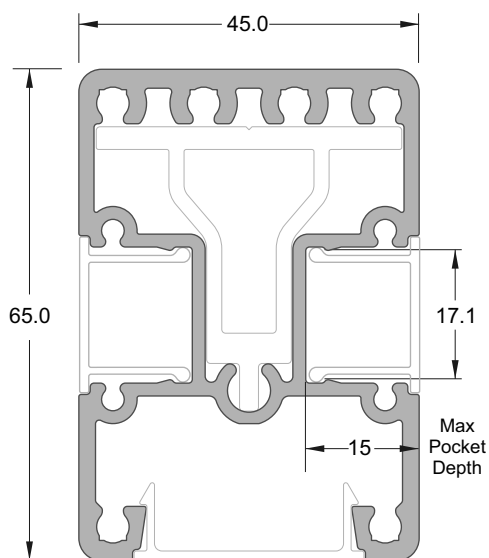
FACE FIX EDGE POST SEMIFRAMELESS JEB/214/5
