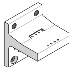
Base plate JEC137/65
