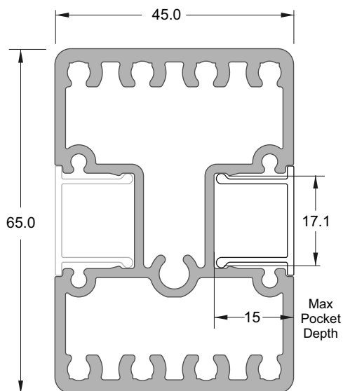
TOP FIX EDGE POST SEMIFRAMELESS JEB/212/5
