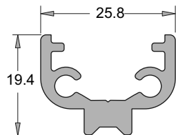
BOTTOM RAIL SPIGOT JVB/017/5
