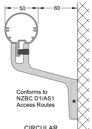
CIRCULAR HANDRAIL JEB/221/5.8
