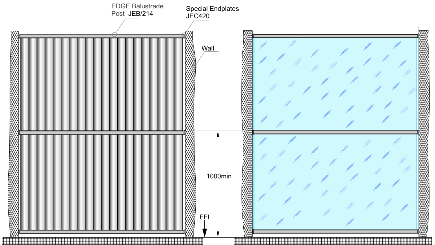
Infill Slat 60mm JVB/019 Gaps 99mm max
