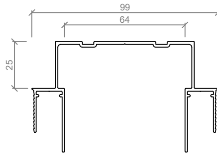
ASL 754 GROOVED HEADSECTION (25mm NEG. DETAIL)
