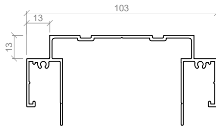
ASL 407 103mm SHADOWLINE HEADSECTION
