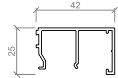
ASL 587 103mm GLAZING BEAD
