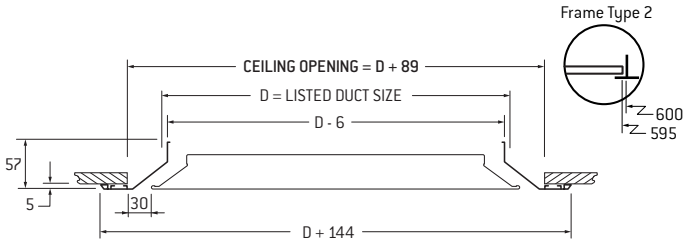
CMPP, Frame Type 1, Surface Mount.
