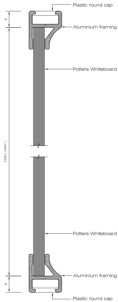
Cross section D - D
