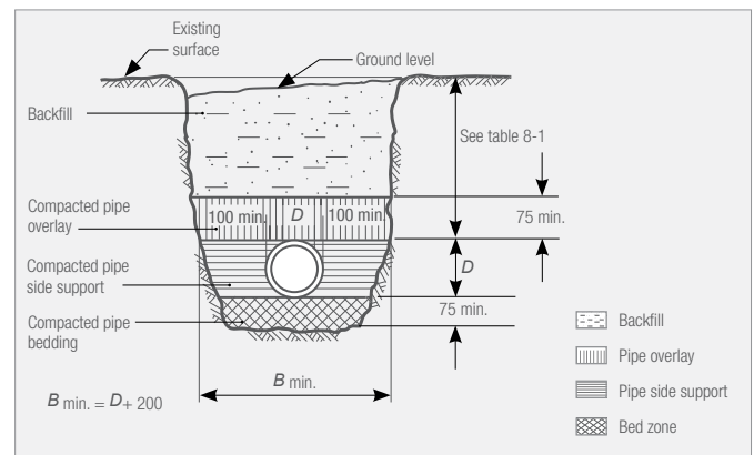
Fig. 8-2 Recommended bedding of drains
