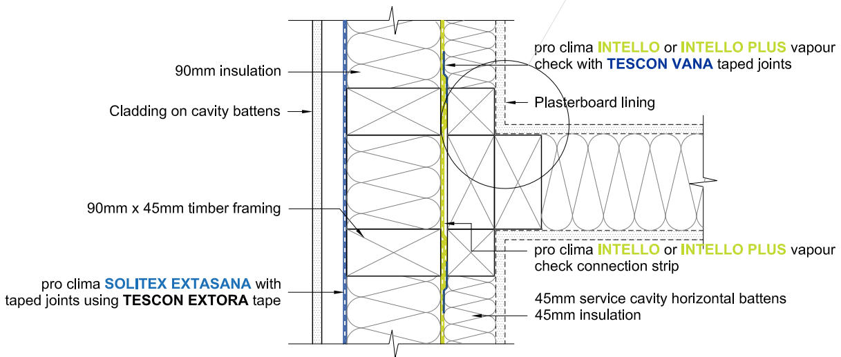
PLANVIEW, 90mm WALL, INTERNAL WALL JUNCTION, WITH SERVICE CAVITY Scale 1:5 @ A4
