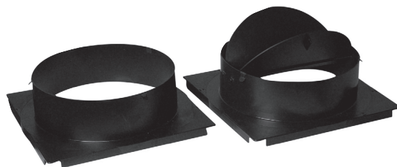
Poly Adaptor & Poly Adaptor with Damper
