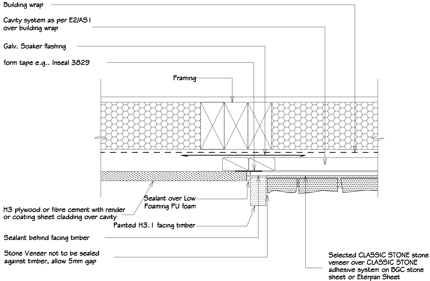
7b - Typical Vertical Joint - Stone Veneer to Plywood or fibre cement sheet with render or coating
