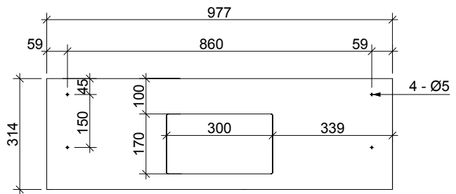
FRAME REAR
