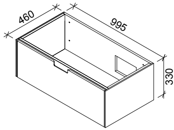
CABINET OVERALL
