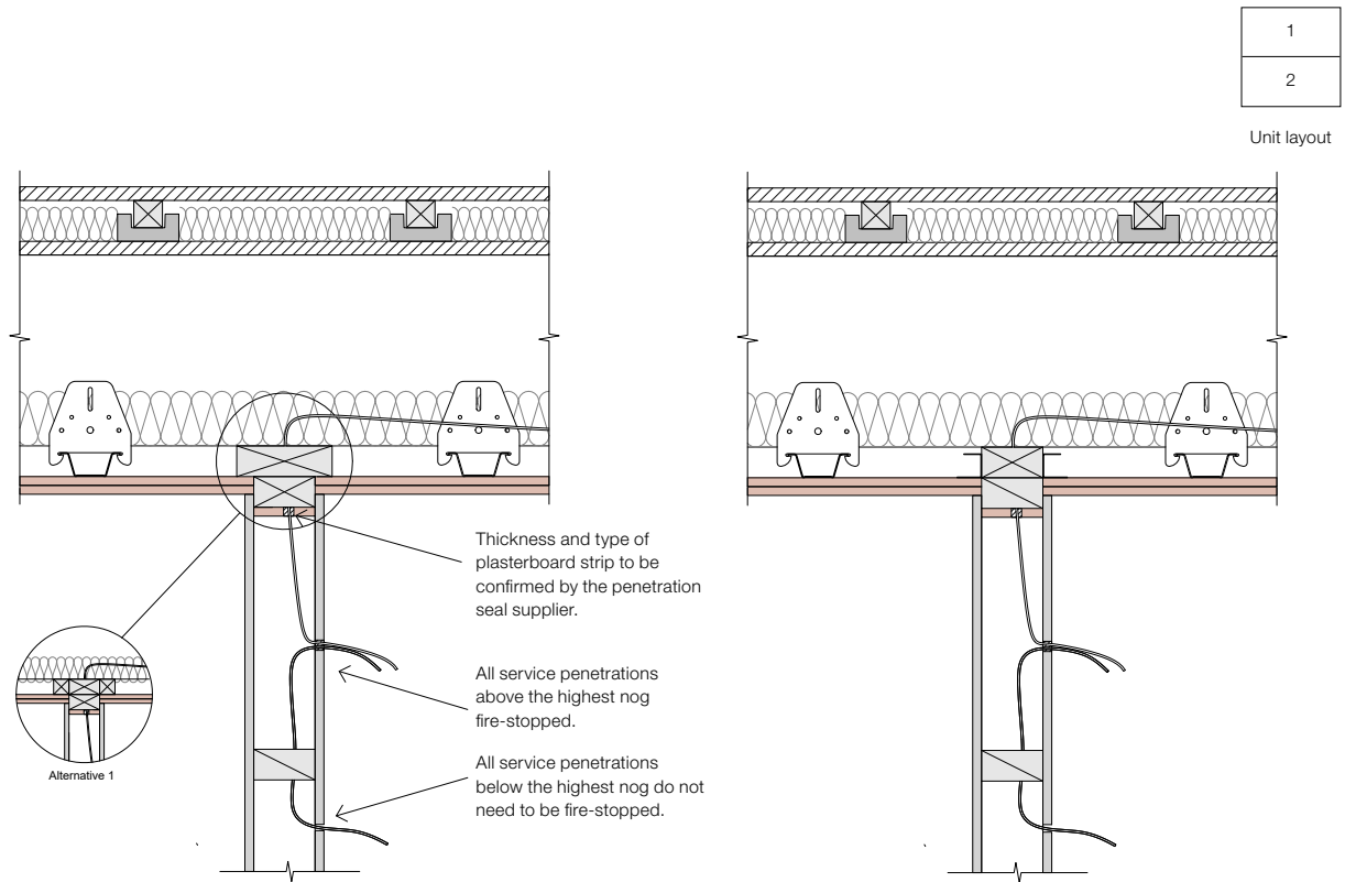
FIGURE 10: NLB Internal Partition or Bracing Wall penetrating the Ceiling Linings both sides, installed in accordance with an FRR no more than 30 minutes less than the floor/ceiling Services fire-stopped using suitable proprietary systems installed below the double top plate Floating floor to mitigate noise flanking
