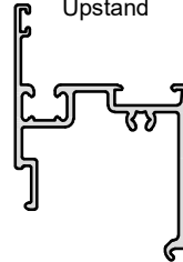
13424NTB Fixed Light Std Upstand
