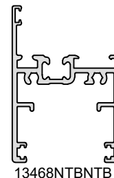
13468NTBNTB Std Beaded Rail
