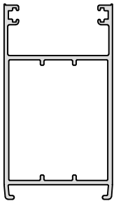
13950 Std Pocketed Lock Stile
