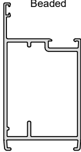
13962 Std Lock Stile Beaded
