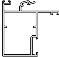
13965 Interlocking Stile Beaded Ext
