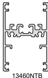
13460NTB Door Narrow Rail / Vision rail
