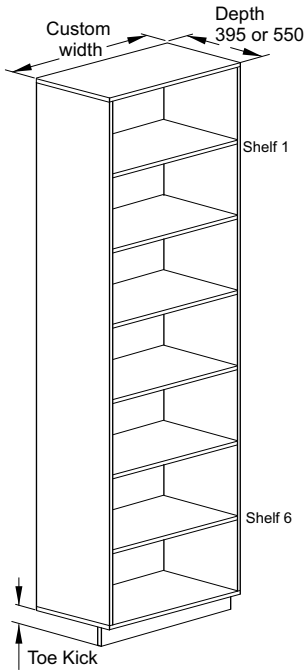
Shelving Unit Wall End shown (either LH or RH)
