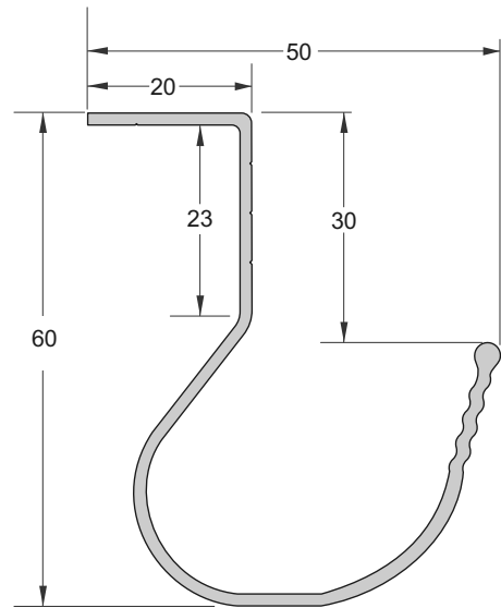
J RAIL CLOSET HANGING TRACK H/8385/4.8
