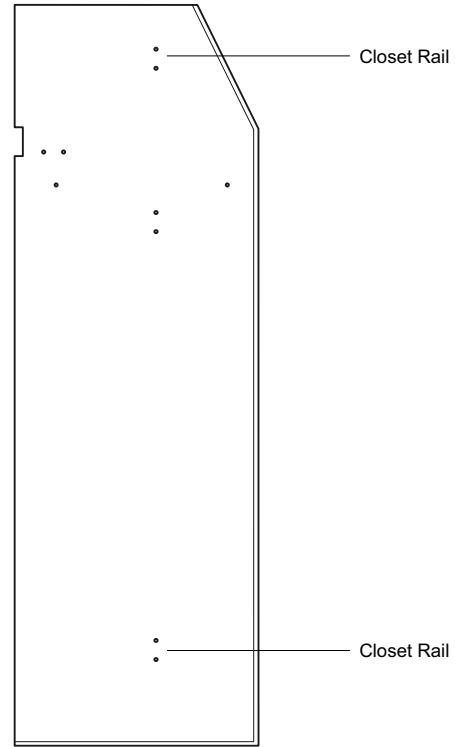
Miter End Panel 1200mm x 395mm
