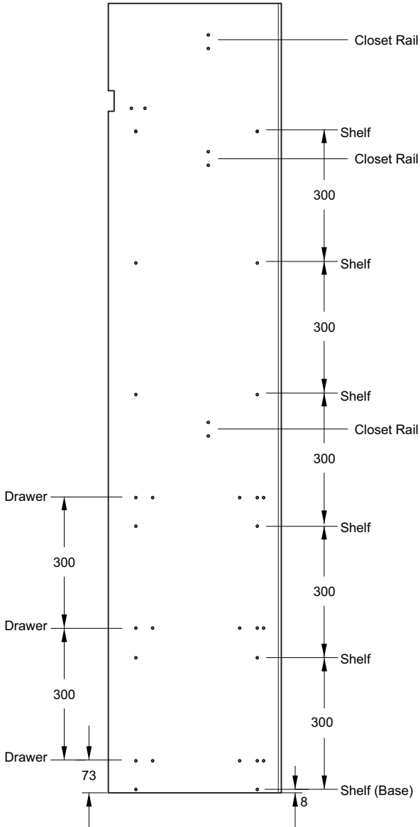
Drilling Layouts Square End Panel 1800mm x 395mm
