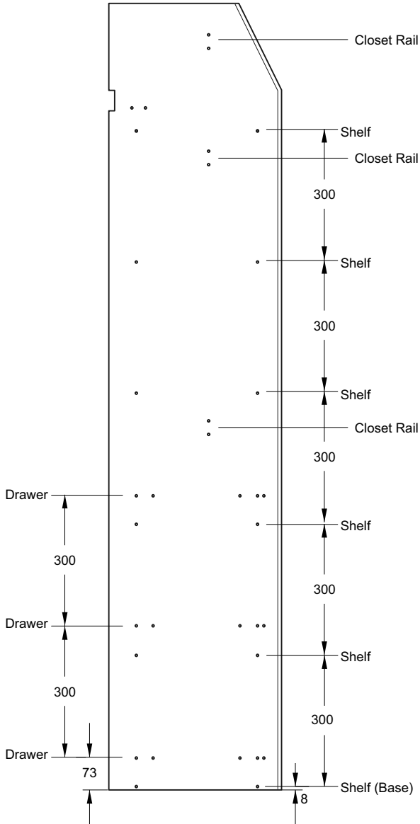
Drilling Layouts Miter End Panel 1800mm x 395mm
