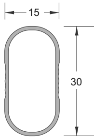
STANDARD CLOSET RAIL H/8384/3
