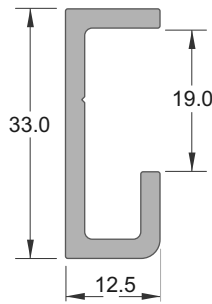
CLOSET HANGING TRACK H/8386/4.8
