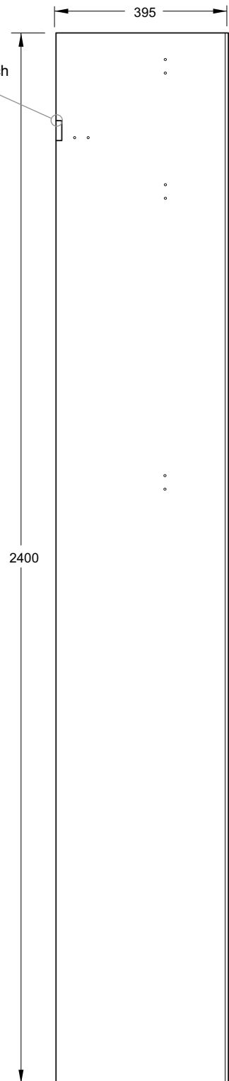
Drilling Layouts Blank Panel 2400mm x 395mm
