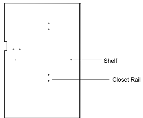
Drilling Layouts Square End Panel 600mm x 395mm
