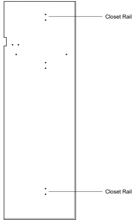
Drilling Layouts Square End Panel 1200mm x 395mm
