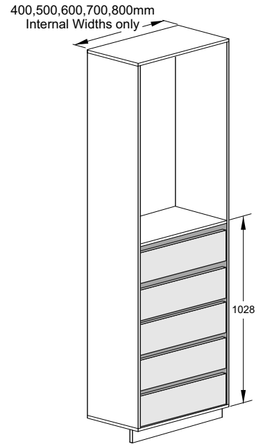
5 x Drawer Unit (Wall Ends shown but any Ends)
