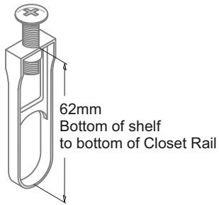
Closet Rail Centre Support H/CO8384CS/CP
