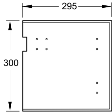
Drilling Layouts Division Panel 300mm x 295mm
