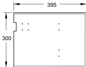
Drilling Layouts Square End Panel 300mm x 395mm
