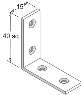
Angle Bracket H/CO8394
