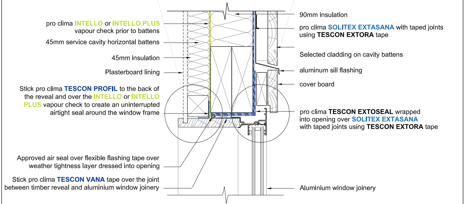
4101 - ELEVATION, 90mm WALL, WINDOW HEAD DETAIL, WITH SERVICE CAVITY Scale 1:5 @ A4
