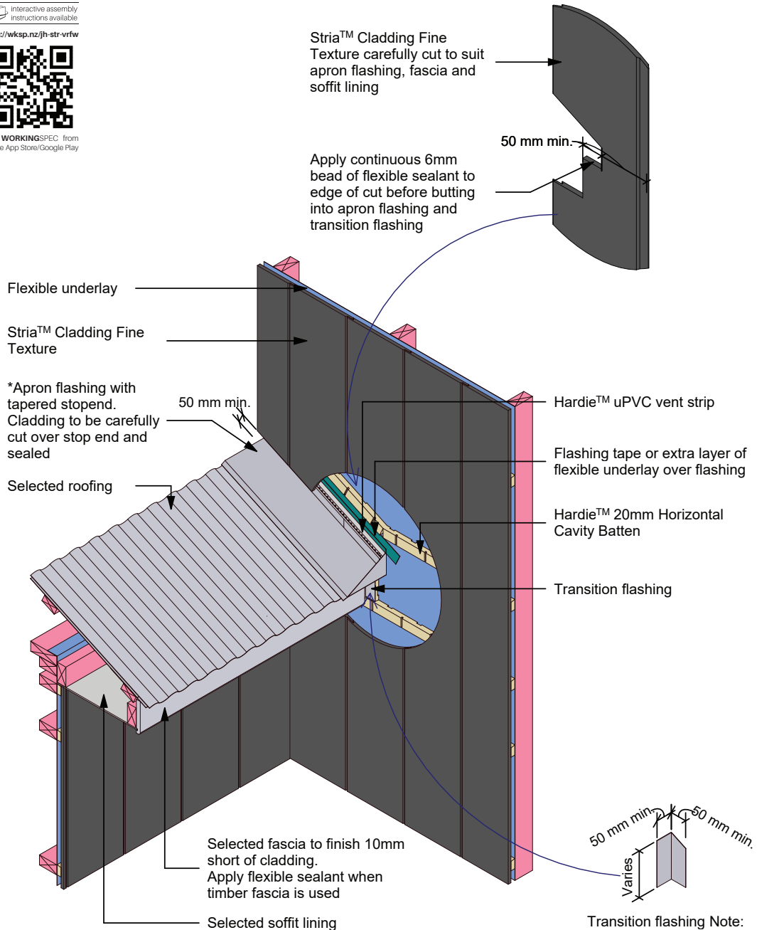
Figure 35: Roof to wall junction
