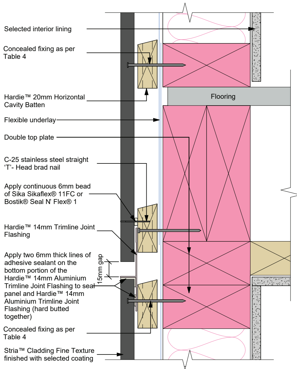
Figure 23: Trimline joint flashing below floor level
