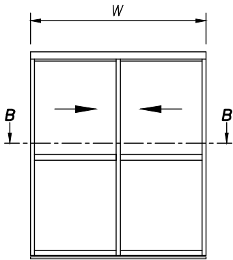
VIEW ON OUTSIDE OF DOOR
