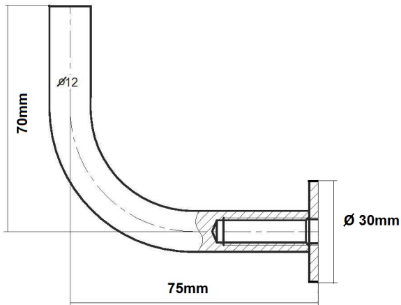
M8 80mm lag screw supplied
