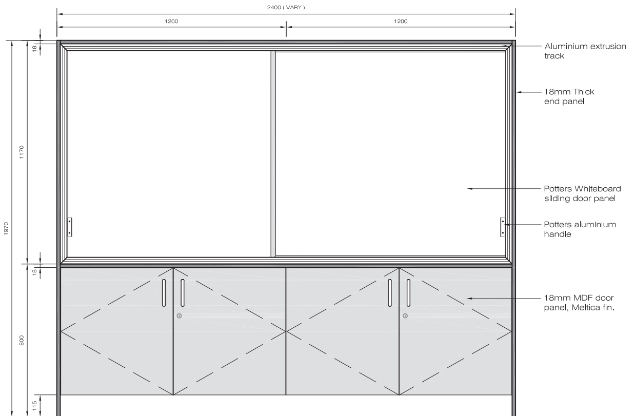
Front elevation - (Storage cabinet)
