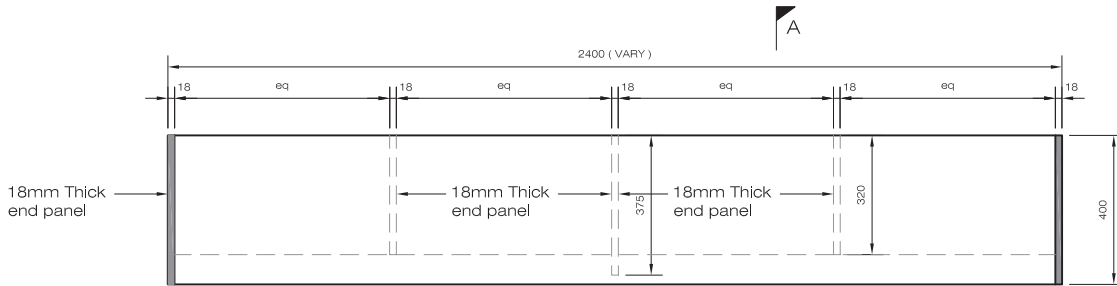
Floor plan - (Storage cabinet)
