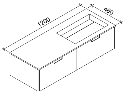
CABINET OVERALL
