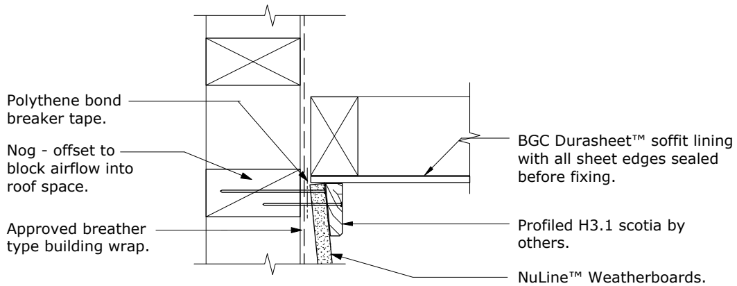
BGC Durasheet™ soffit/Nuline Weatherboards
