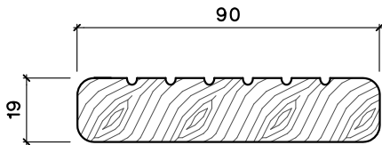
J6 Decking 90x19
