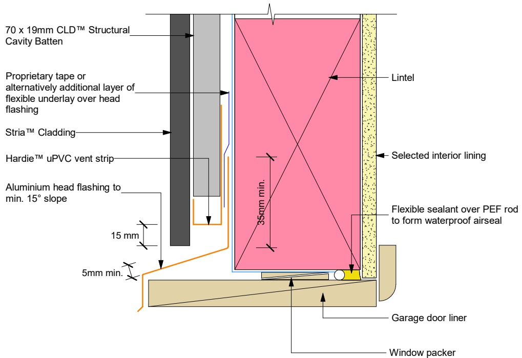
Figure 37: Garage head
