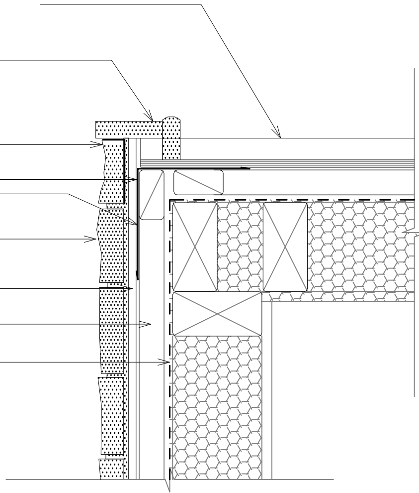
6a - Typical External Corner with Plywood Cladding
