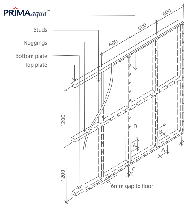
Figure 2: Vertical sheet fixing
