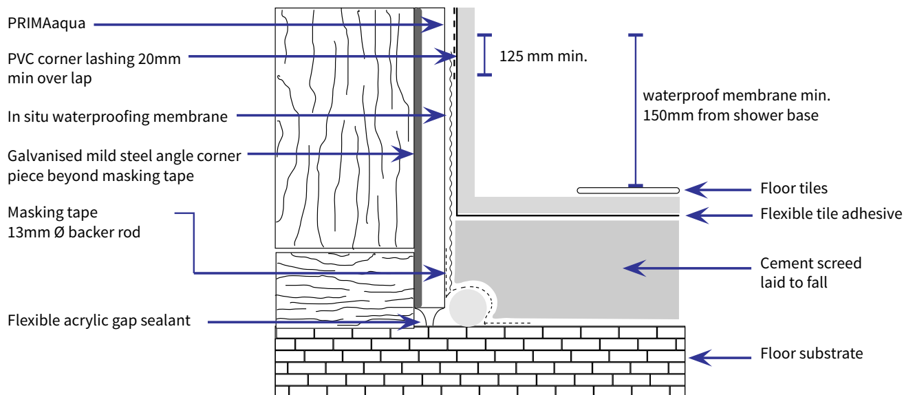
Typical floor / wall cross-section for cast in-situ internal membrane
