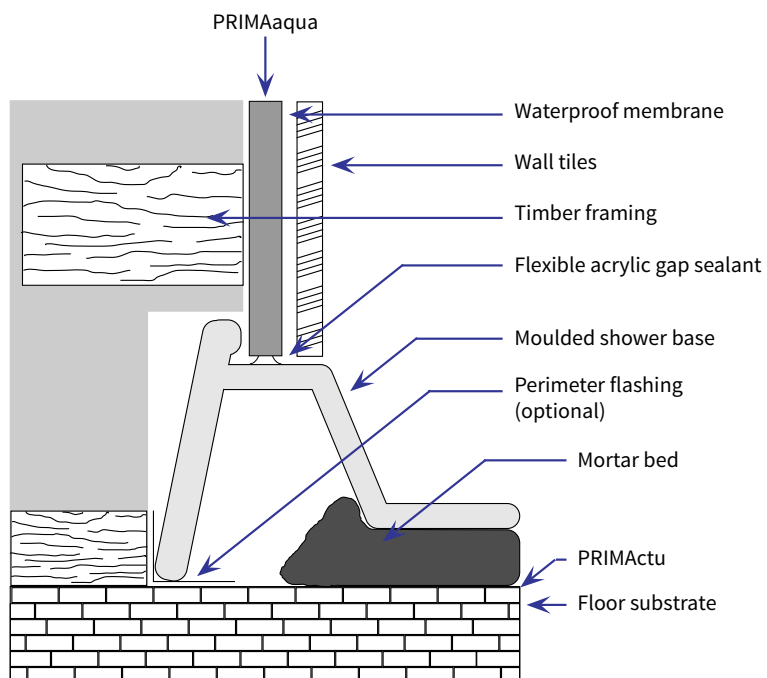
Typical detail at shower recess
