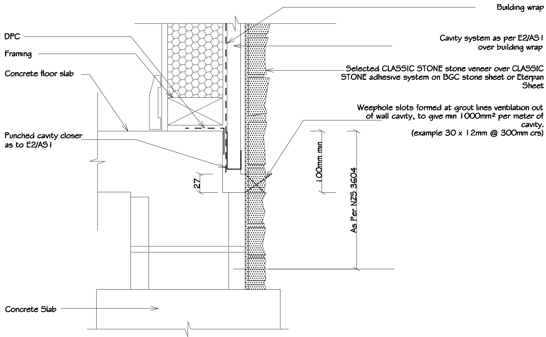
9a - Typical Rebated Slab Edge Detail
