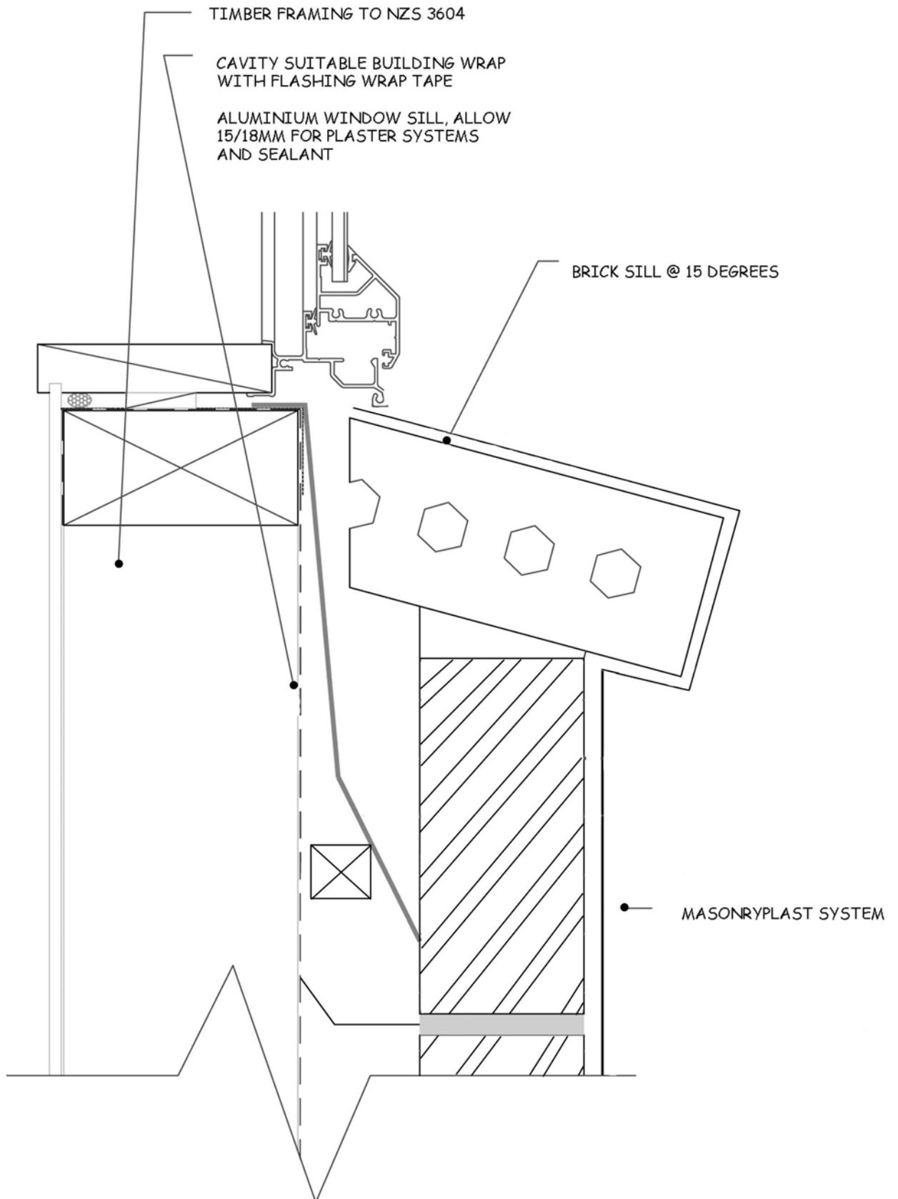
02 SILL DETAIL
