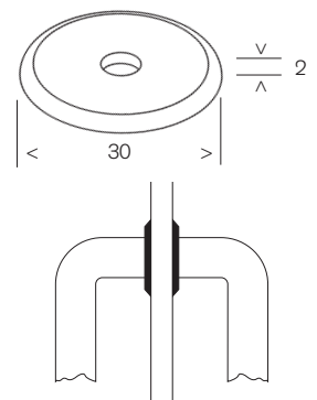
MW30 Gold Highlight Washer To suit MK25 Knob Set and MS and M250 Handles
