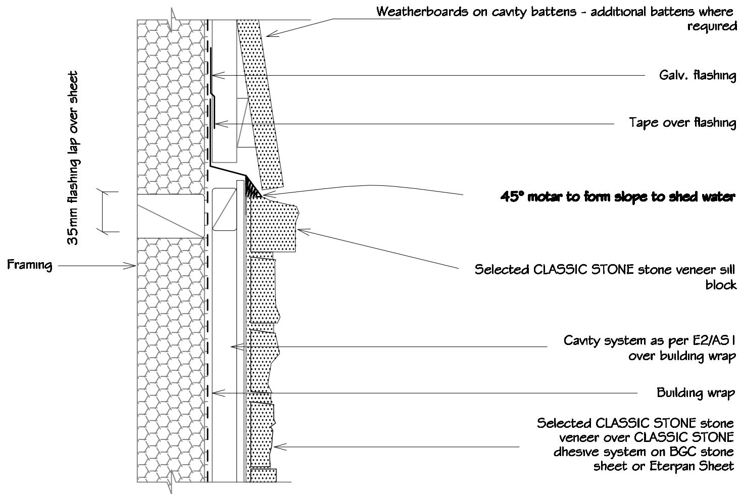
1c - Typical Horizontal Joint with Weatherboard - Cavity
