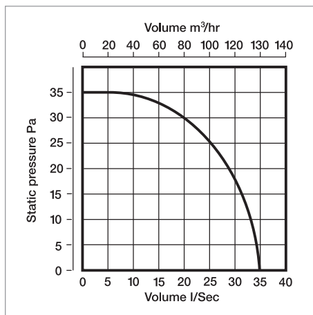
Performance - XFLP125
