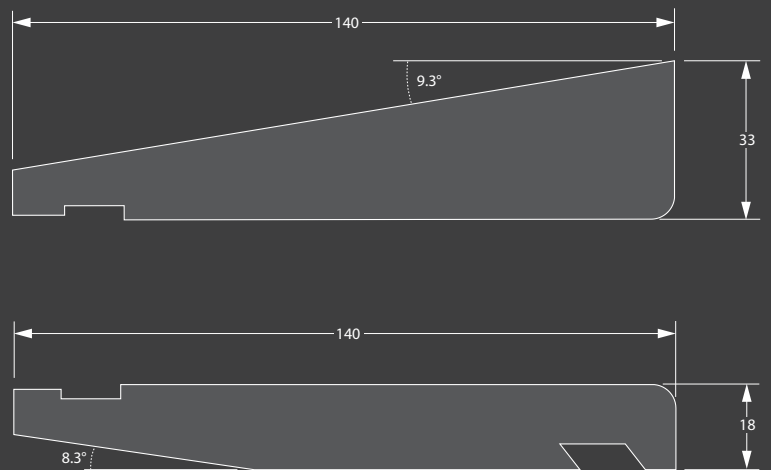
140mm Bevelback SmartClad weatherboards Top — 140mm Starter Board. Above — 140mm Weatherboard profile
