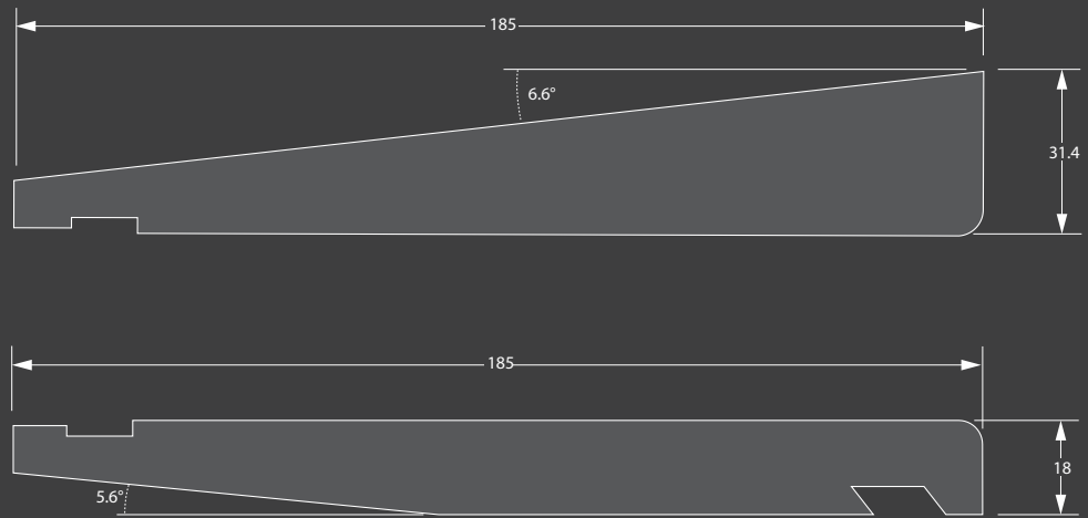
185mm Bevelback SmartClad weatherboards Top — 185mm Starter Board. Above — 185mm Weatherboard profile
