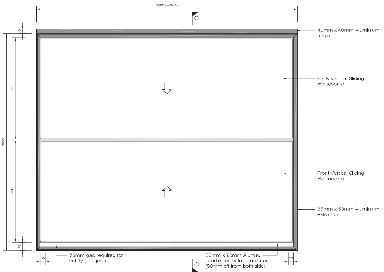
Front elevation - (Counterbalance)
