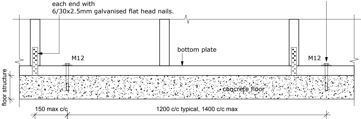
Brace Panel Hold Down - Construction Detail BGC - DS3 (1200mm) & DS4 (2400mm) Concrete Floor
