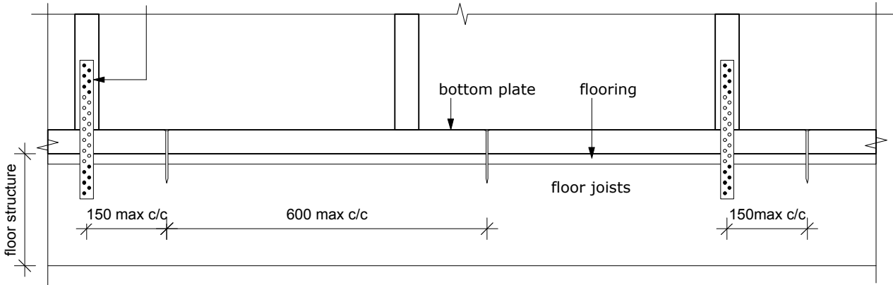
Brace Panel Hold Down - Construction Detail BGC - DS1 (1200mm) & DS2 (2400mm) Timber Floor
