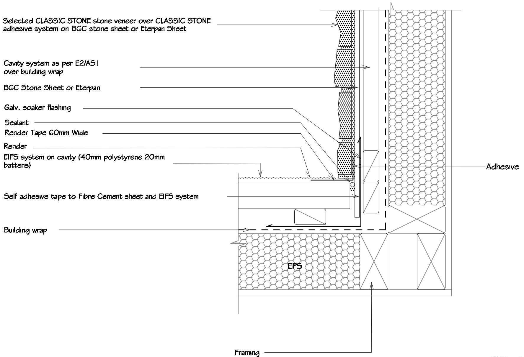
5c - Typical Internal Corner with EIFS Cavity System (plan view)
