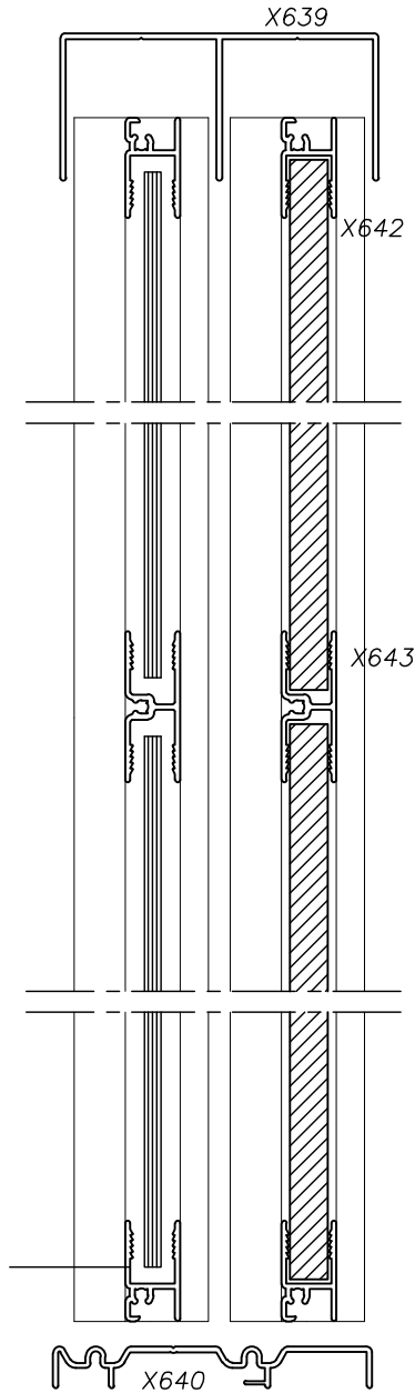
SECTION AA
