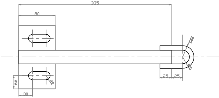
SE005A Roof Anchor Plan Scale 1:1
